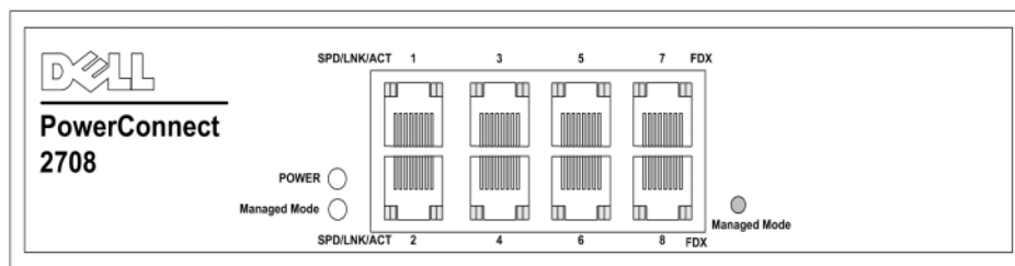
Figura 1-1. Panel frontal de PowerConnect 2708
